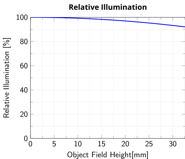
Relative illumination vs. Object Field Height, from the optical axis to the corner of the field of view, wf/N = 8
