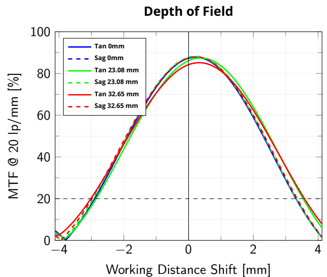
Modulation Transfer Function (MTF) @ 20 lp/mm vs. Working Distance Shift from the best focus Working Distance, wavelength range 440-640 nm, wf/N = 8
