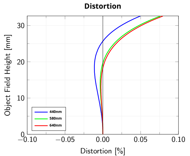
Object Field Height vs. Distortion, from the optical axis to the corner of the field of view, wf/N = 8
