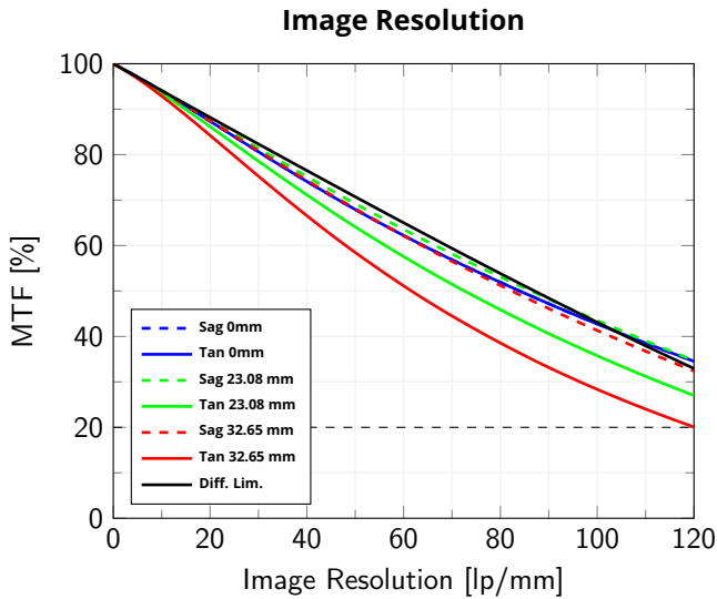
Modulation Transfer Function (MTF) vs. Image Resolution, wavelength range 440-640 nm, wf/N = 8
